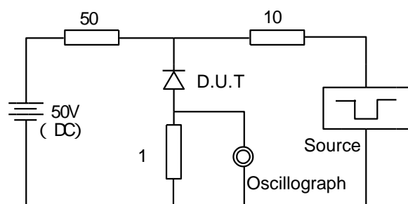
TEST CIRCUIT AND REVERSE RECOVERY TIME WAVEFORM .
