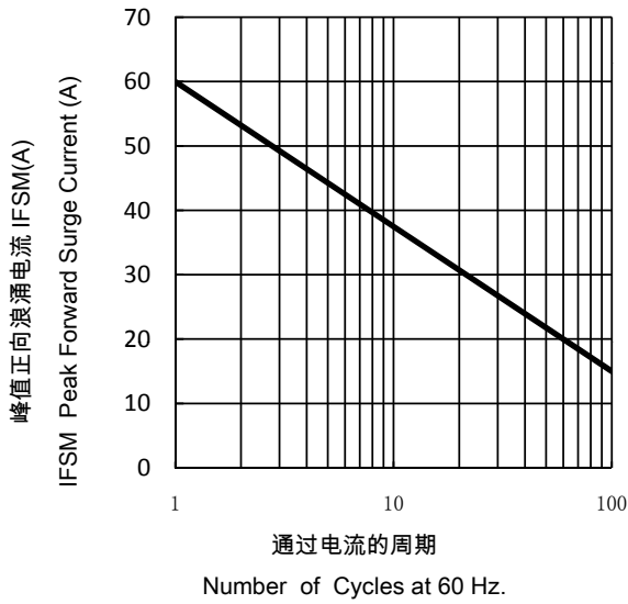
Non Repetitive Peak Forward Surge Current
