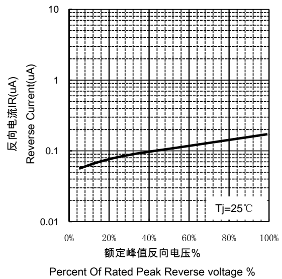
反向特性曲线 TYPICAL REVERSE CHARACTERISTICS
